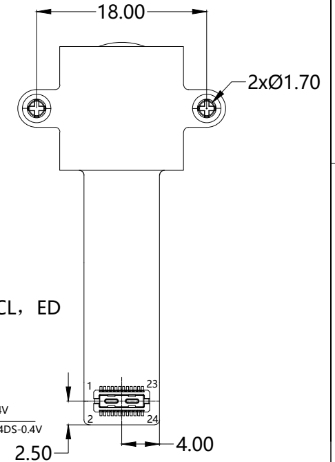
BOTTOM VIEW
